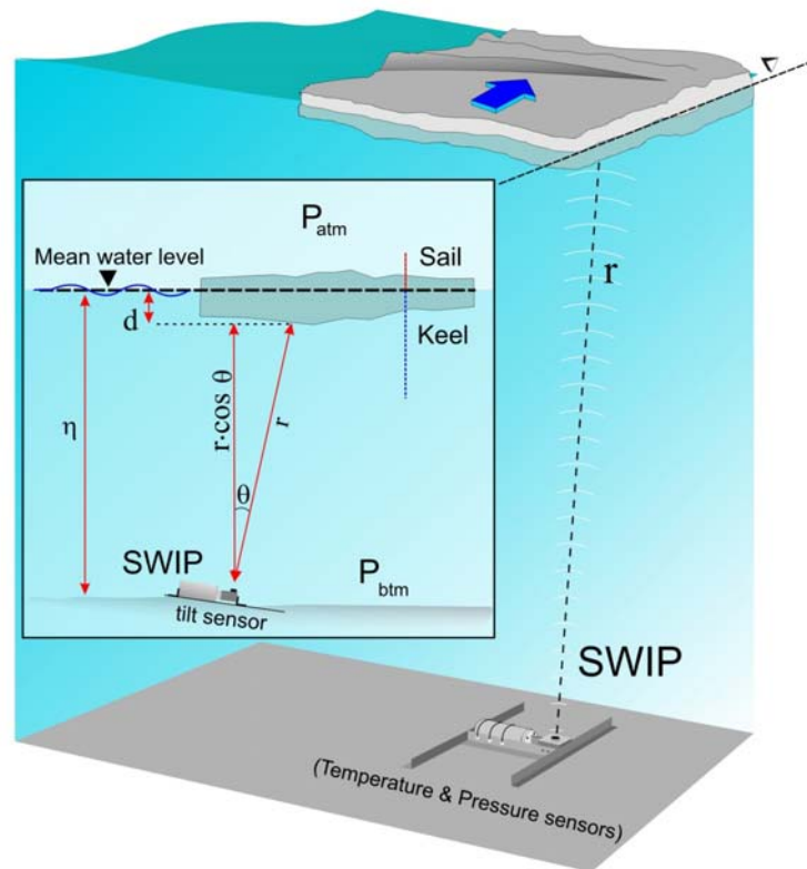
Figure 1. SWIP configuration and measurements parameters are shown above.
